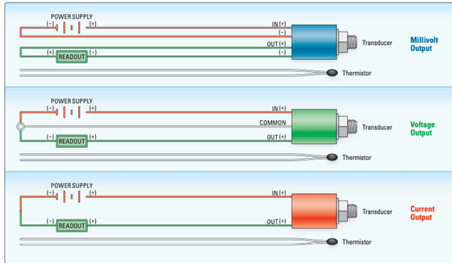
• Model 3400 Series Semiconducting Piezometer wiring schematics.
